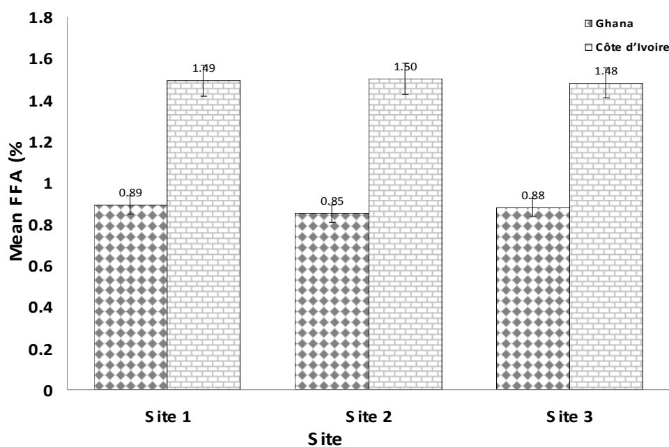
Fig. 3 FFA contents of 2008 crop year cocoa beans from Ghana and Cote d'Ivoire.
