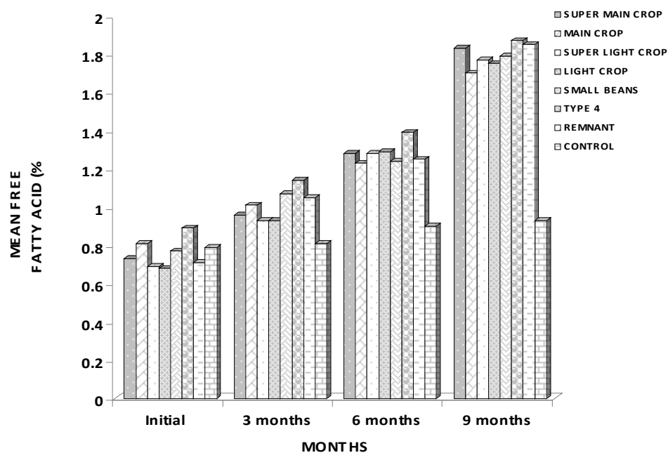
Fig. 2 FFA contents of various categories of dry cocoa beans from Ghana artificially infested with stored product insects and stored over different periods of time (s.e. = 0.006).
