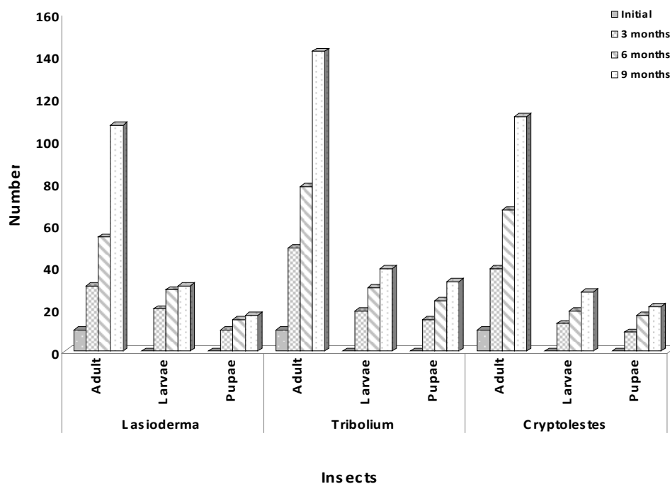
Fig. 1 Number of insects found on 500 g of dry cocoa beans from Ghana after various months of storage (s.e. = 0.044).
